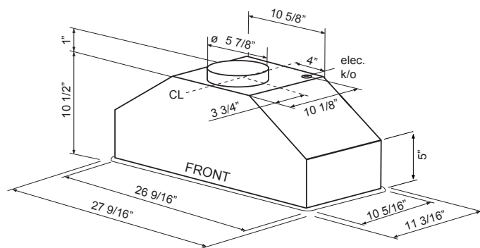
Cabinet Bottom Cut-Out Size (W x D): 26 3/4" x 10 1/2"
