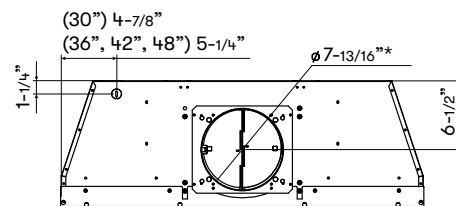
REAR
