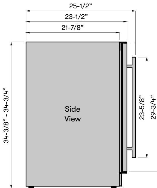
*For flush-mount cabinet installations
