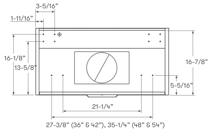
Back View Mounting Dimensions
