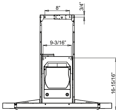
Back of Hood
