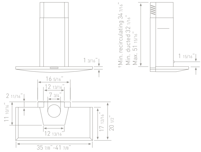
† Ductless (Recirculating); lower holes exposed. Note: if necessary order the proper duct cover extension kit.
